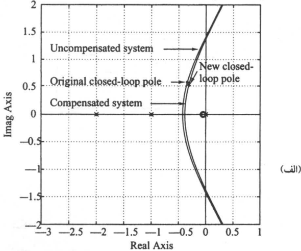
Root-Locus Plots of Compensated and Uncompensated Systems
